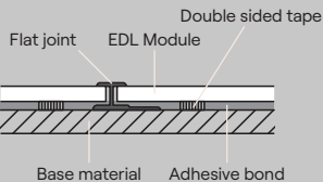
Flat joint
