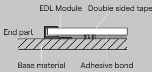
End part
