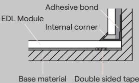
Internal corner
